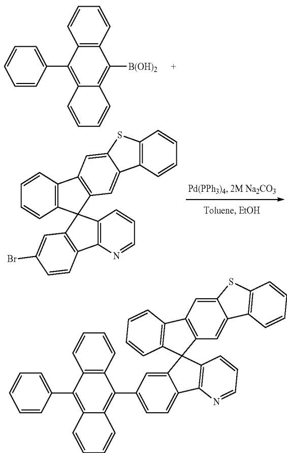
Compound 2
