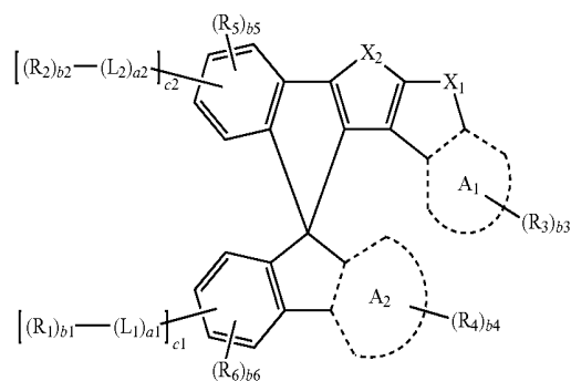
Formula 1D
