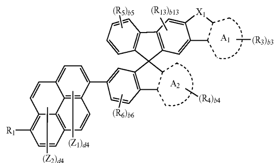
Formula 1A-2
