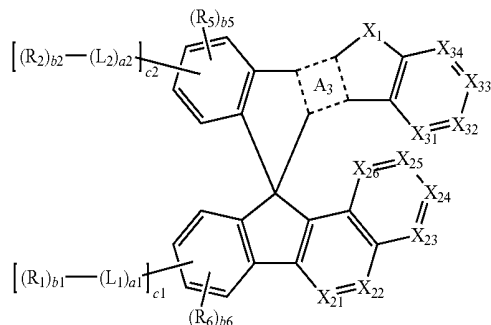
Formula 1-7
