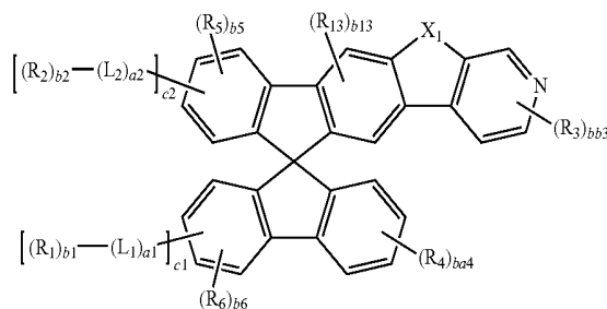
Formula 1(7)
