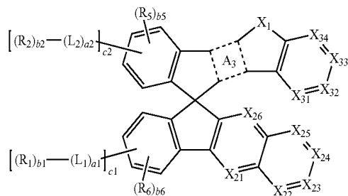
Formula 1-7
