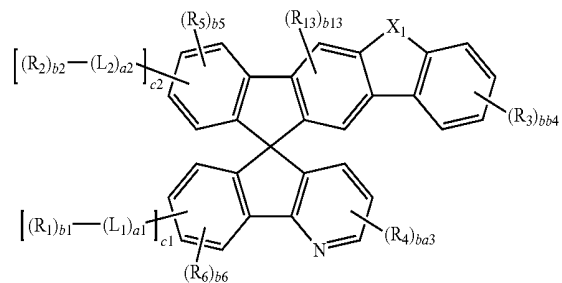
Formula 1(3)
