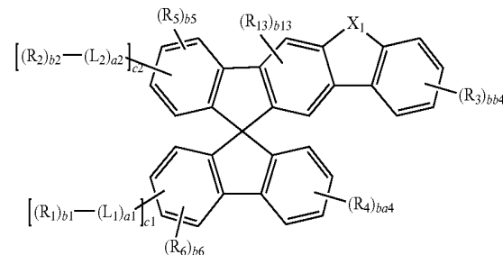
Formula 1(2)
