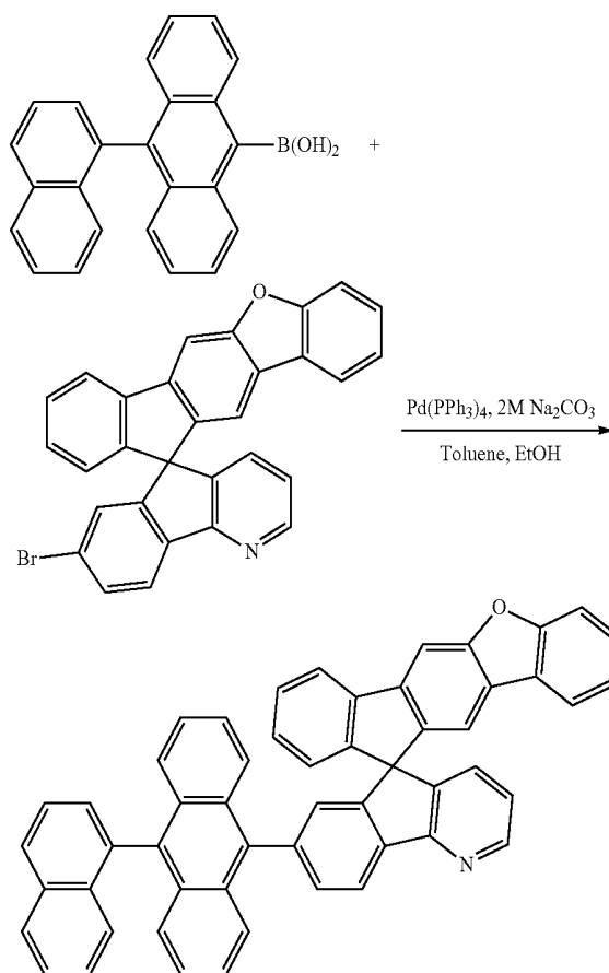
Compound 7
