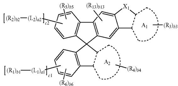
Formula 1B
