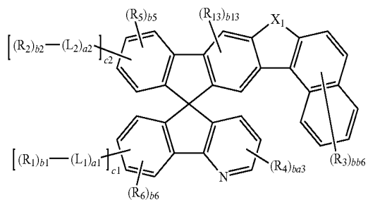
Formula 1(22)
