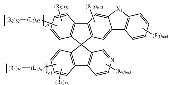
Formula 1(6)
