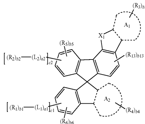
Formula 1C
