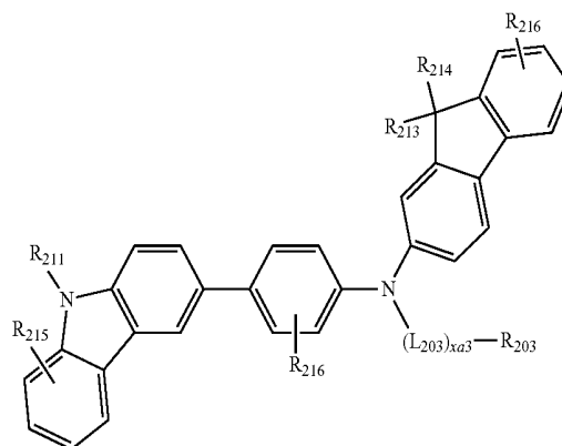
Formula 201A-1
