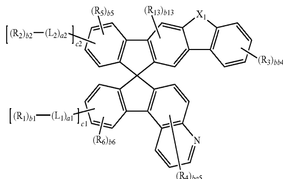
Formula 1(10)
