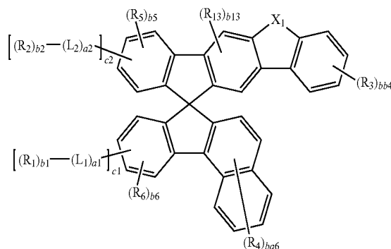
Formula 1(9)
