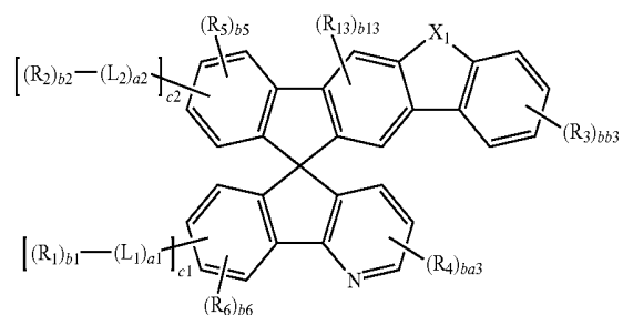
Formula 1(4)
