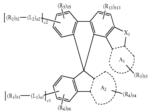
Formula 1C
