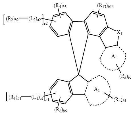
Formula 1D
