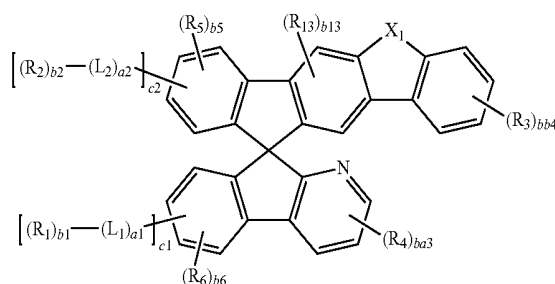
Formula 1(8)
