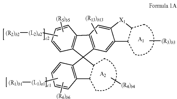
Formula 1A
