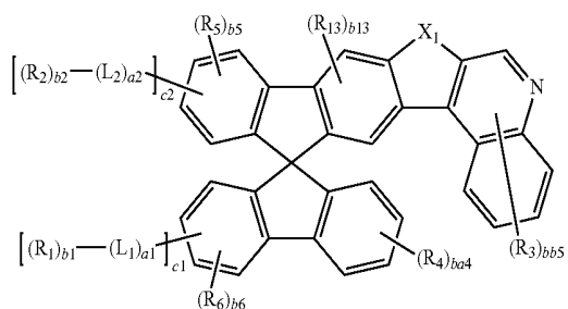
Formula 1(21)
