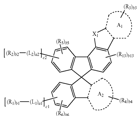
Formula 1B
