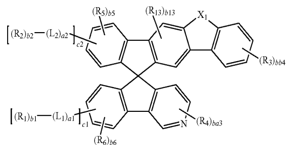
Formula 1(5)
