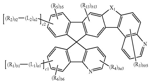
Formula 1(23)
