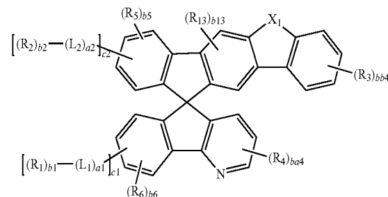
Formula 1(3)
